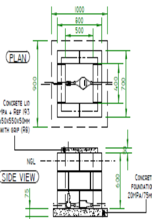
E CHAMBER FOR GATE VALVE & WATER METER
